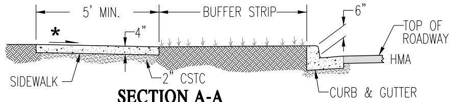
SIDEWALK RAMP TYPE 3A
