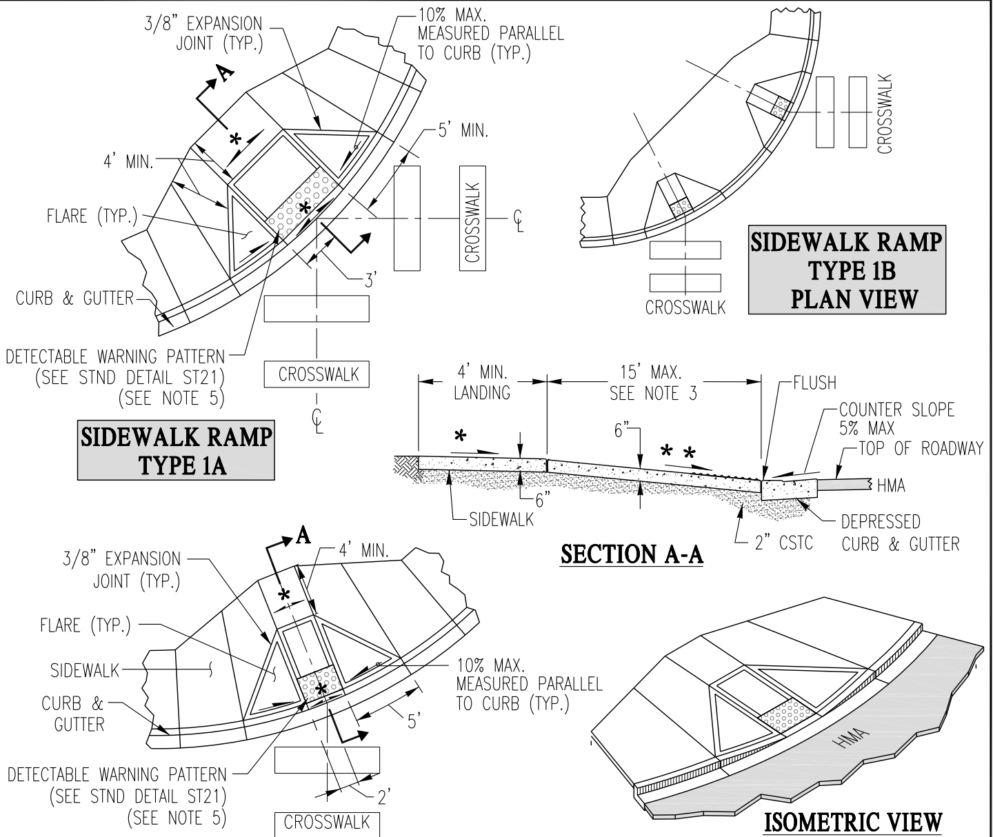
SIDEWALK RAMP TYPE 1B
