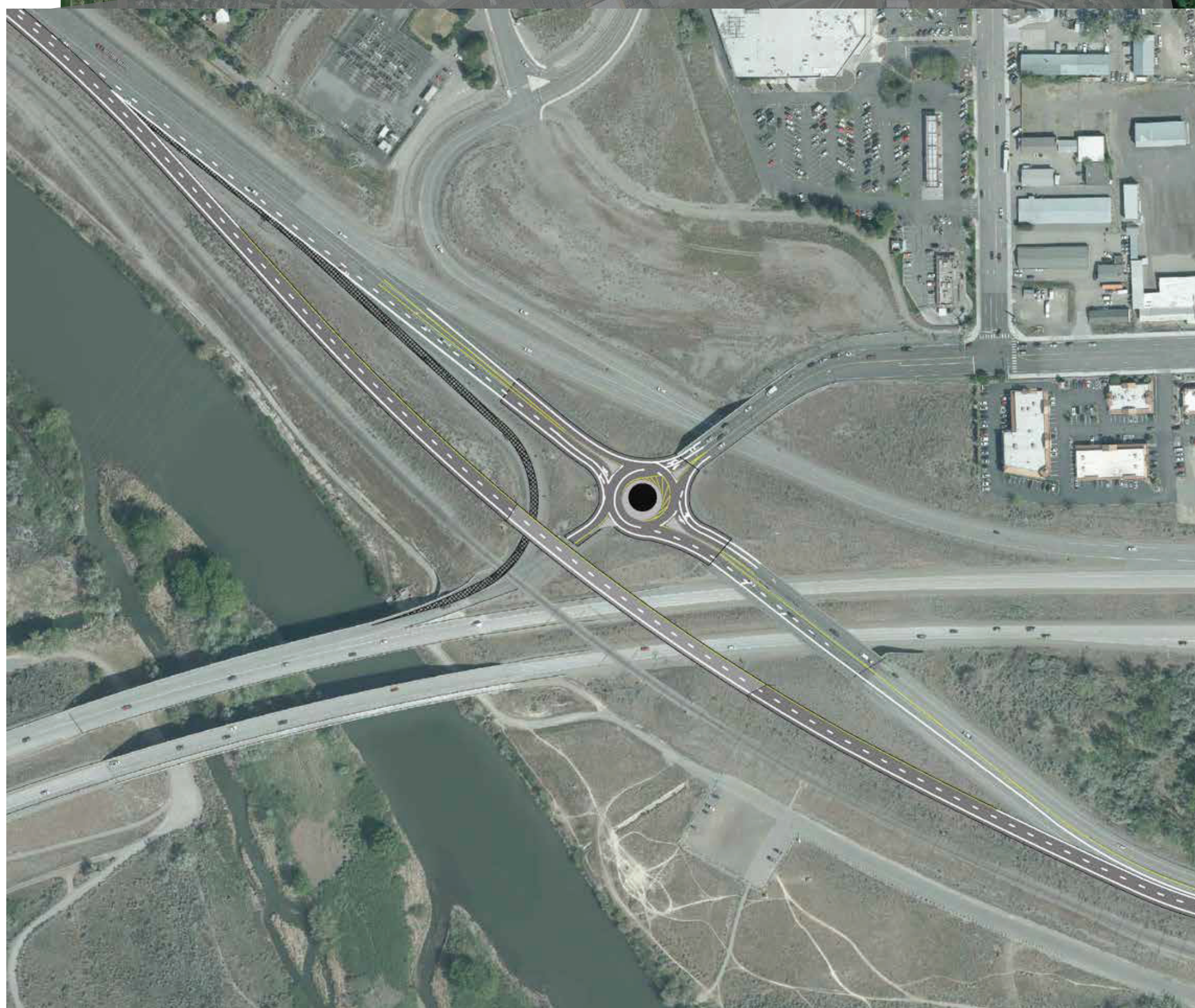
Detail of Aaron Drive Interchange
